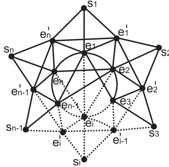
Fig.4 Line Graph of Helm Graph L(H_n)
