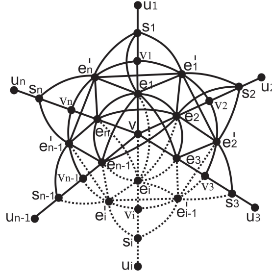
Fig.5 Middle Graph of Helm Graph M(H_n)
