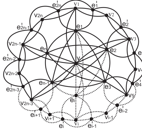
Fig.9 Total graph of Gear Graph T(G_n) .
