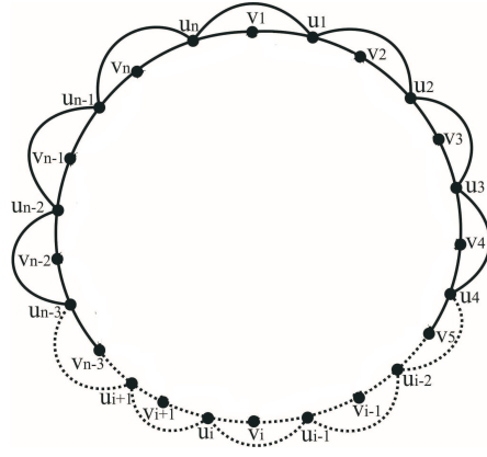
Fig.1 Middle Graph of Cycle M(C_n)
