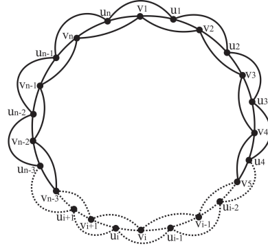
Fig.2 Total Graph of Cycle T(C_n)
