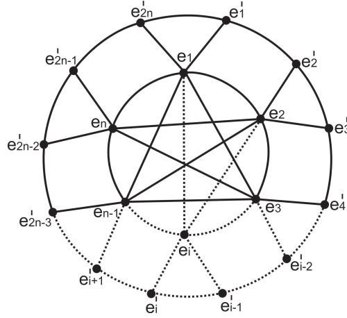
Fig.7 Line graph of Gear Graph L(G_n) .
