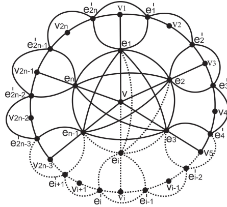
Fig.8 Middle graph of Gear Graph M(G_n) .
