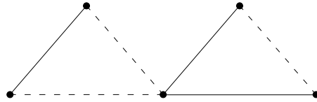
Fig.1 Net-regular signed graph \Sigma_5^0 for C_3
