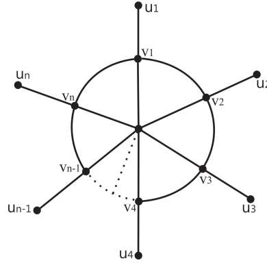
Fig.3 Helm Graph H_n
