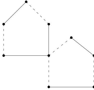
Fig.2 Net-regular signed graph \Sigma_7^0 for C_4
