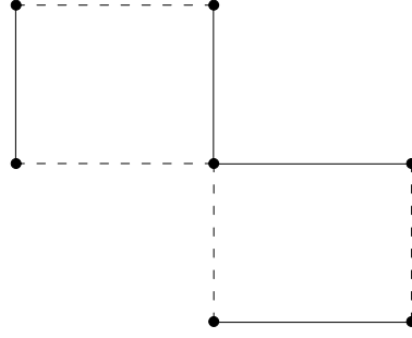
Fig.2 Net-regular signed graph \Sigma_7^0 for C_4
